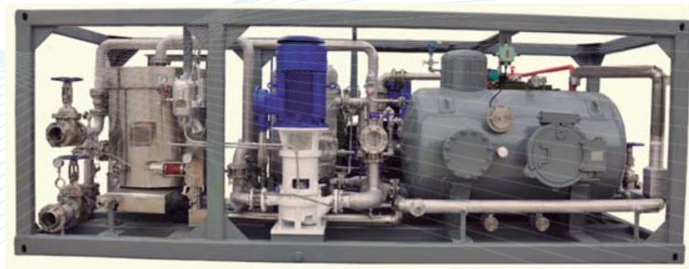
Mobile Automatic Cleaning Unit of Oil-storage Tanks
